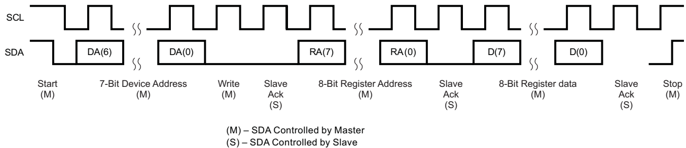
Figure 31. I²C Write
