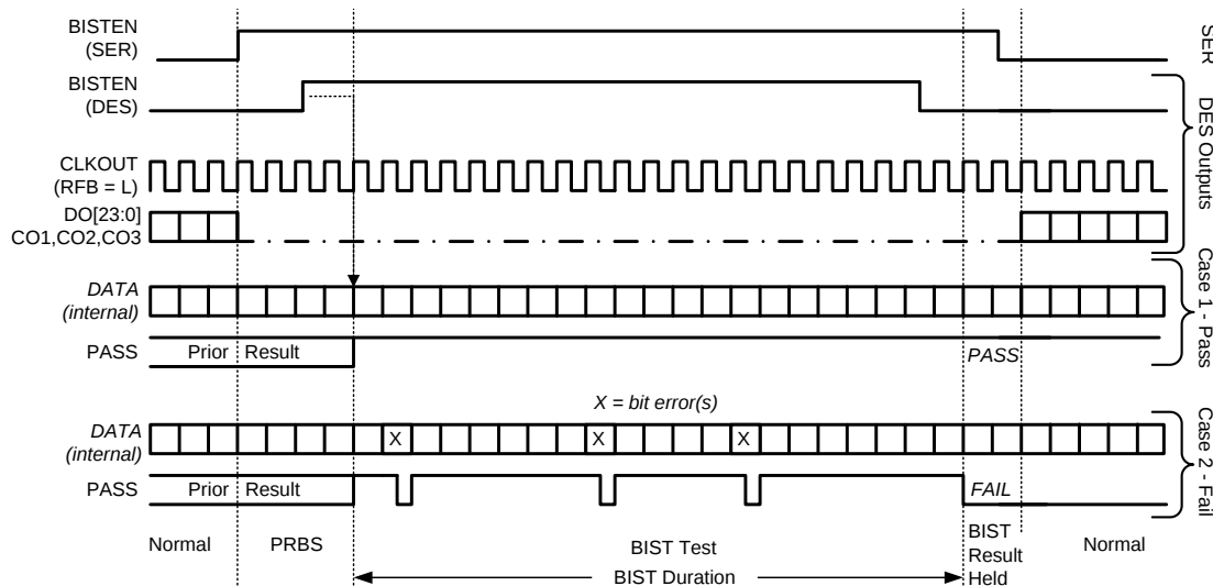
Figure 29. BIST Waveforms
