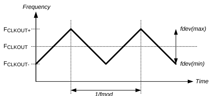
Figure 22. SSCG Waveform
