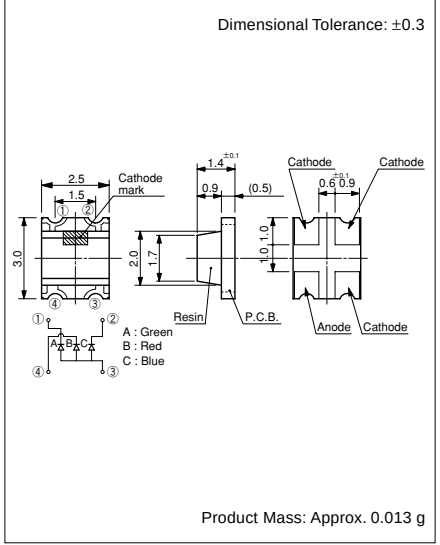
External Dimensions (Unit: mm)
