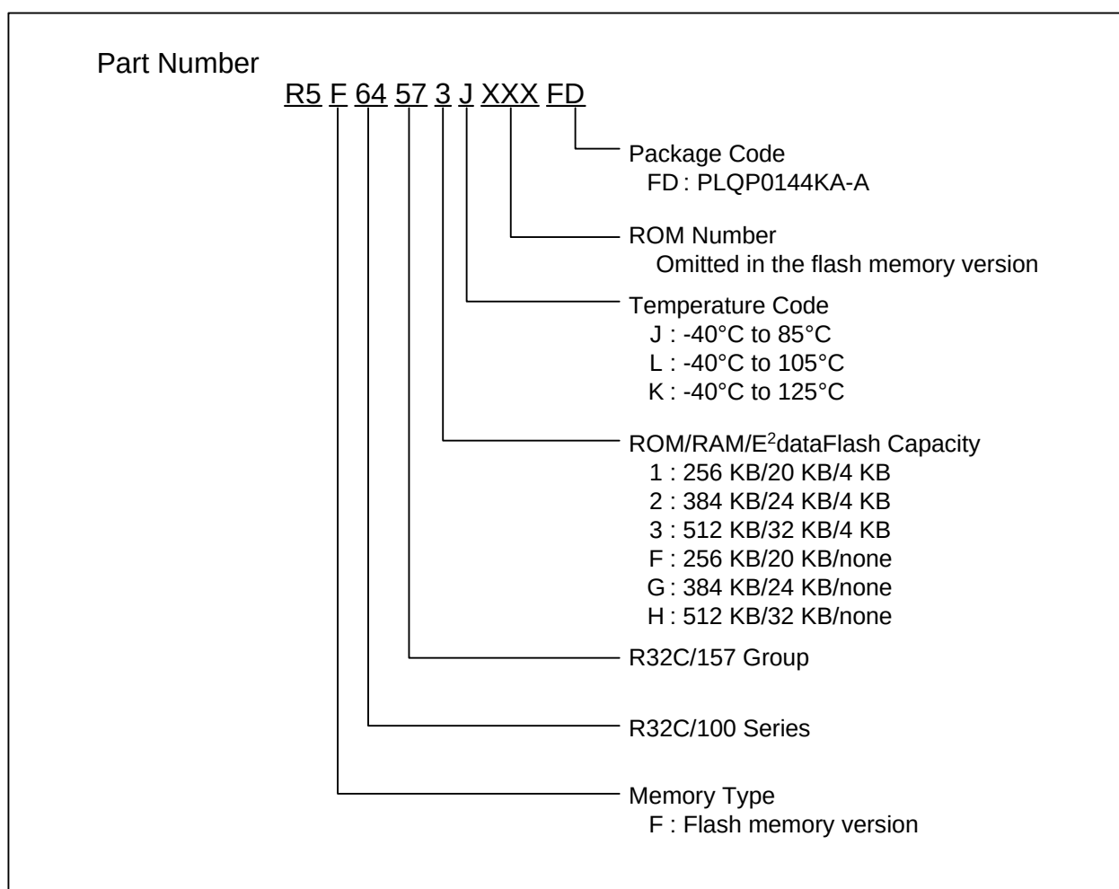
Figure 1.1 Part Numbering
