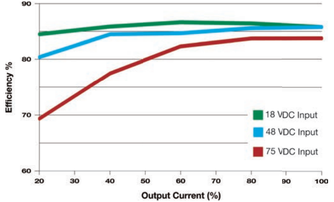
Efficiency vs Output Load: 48 VIN Models
