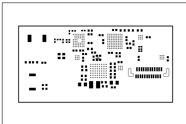
MAX32620UCBLEEK#—Top Paste
