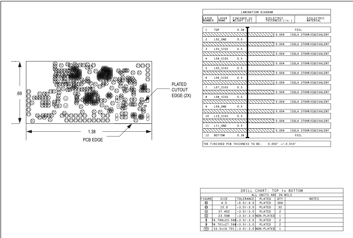
MAX32620UCBLEEK#—Fab Notes
