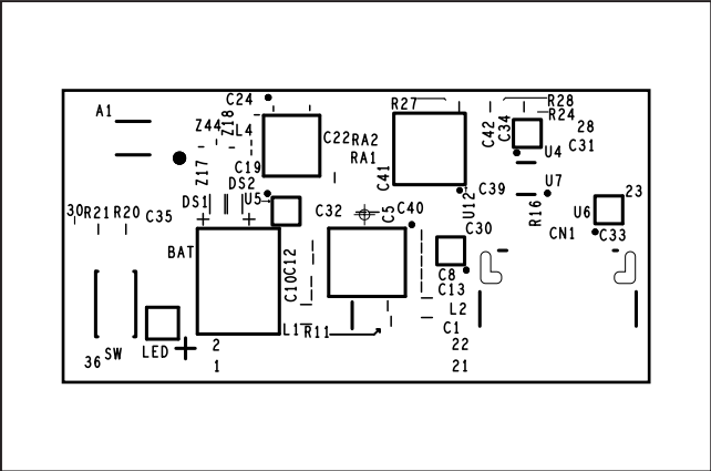
MAX32620UCBLEEK#—Top Silkscreen
