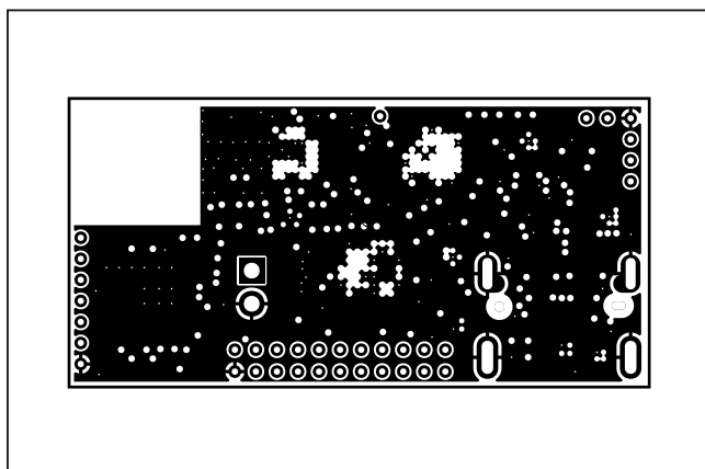
MAX32620UCBLEEK#—L11 GND
