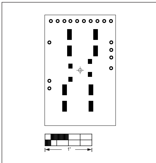
MAX86141OSBEK#—Bottom
