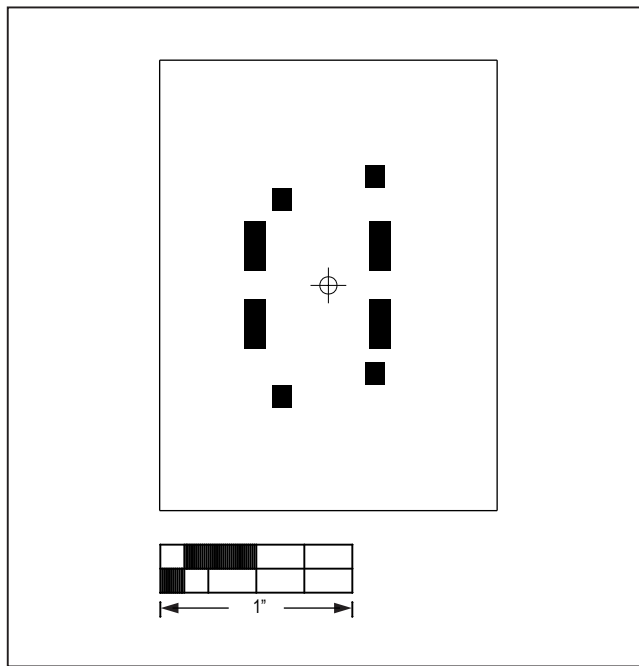
MAX86140OSBEK#—Bottom Paste
