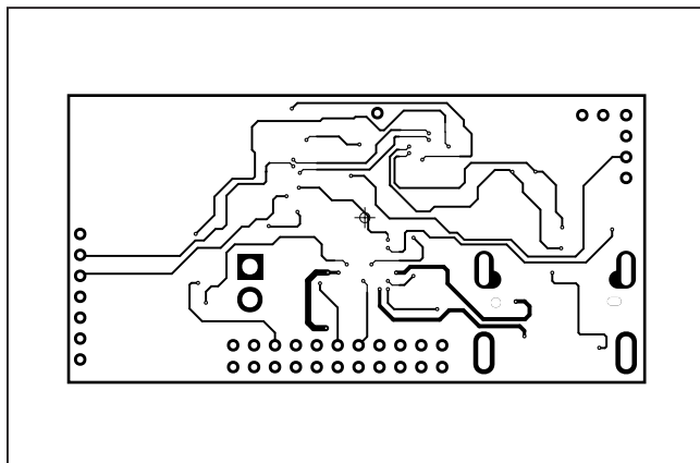
MAX32620UCBLEEK#—L08 SIGS
