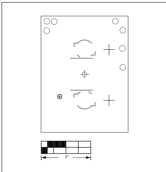
MAX86140OSBEK#—Bottom Silkscreen
