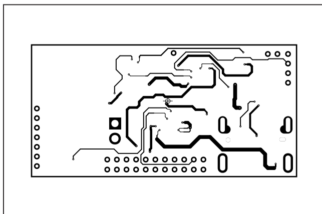
MAX32620UCBLEEK#—L07 SIGS
