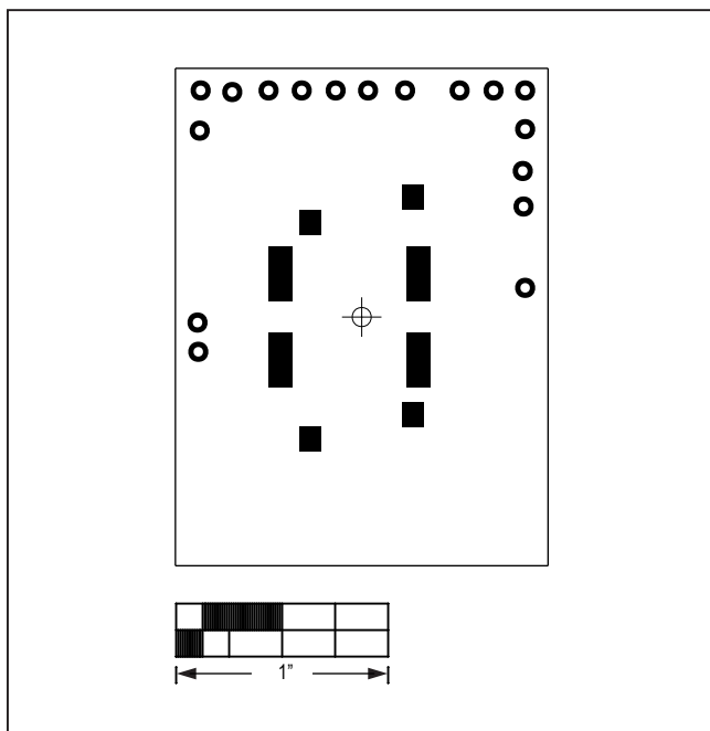
MAX86140OSBEK#—Bottom Mask
