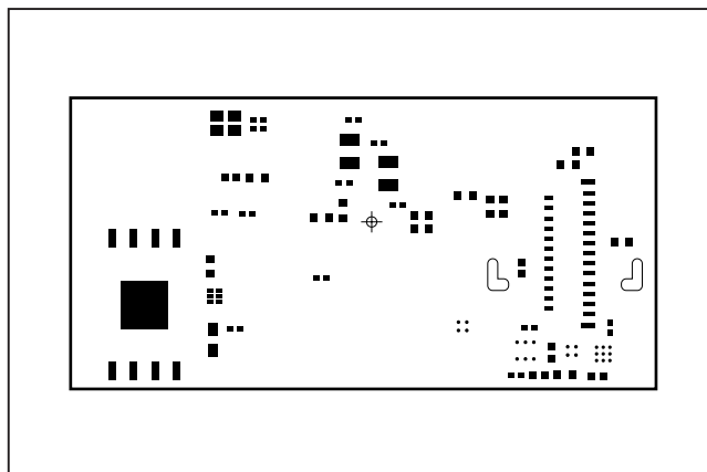
MAX32620UCBLEEK#—Bottom Paste
