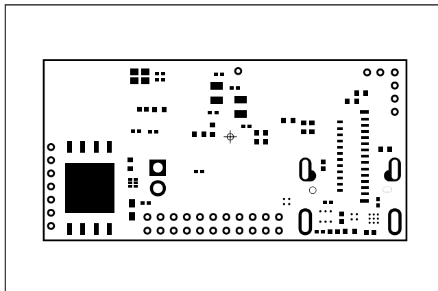
MAX32620UCBLEEK#—Bottom Mask
