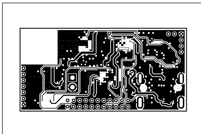
MAX32620UCBLEEK#—L04 SIGS
