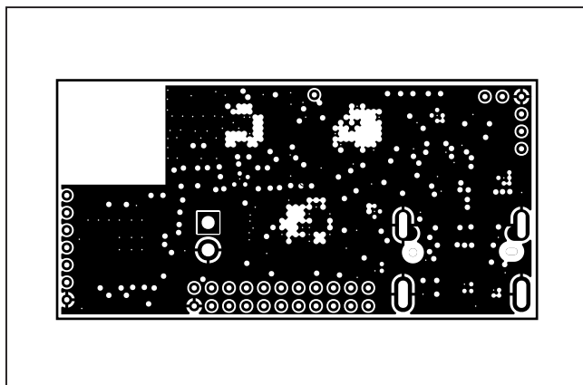
MAX32620UCBLEEK#—L2 GND
