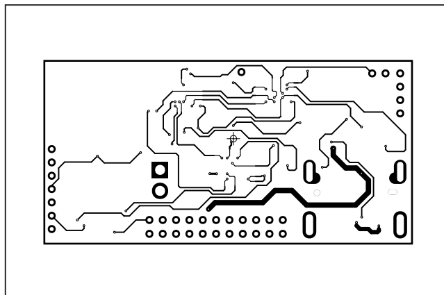
MAX32620UCBLEEK#—L03 SIGS
