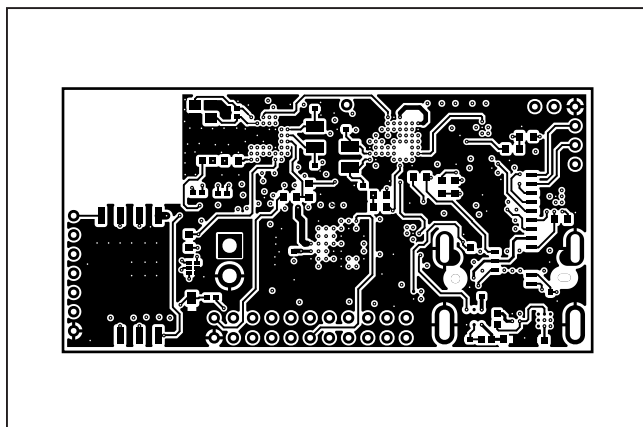
MAX32620UCBLEEK#—Bottom
