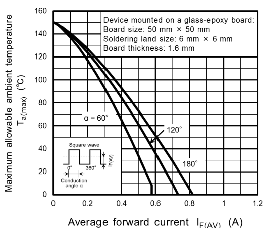
Fig. 10.4 T_{a(max)} - I_{F(AV)}
