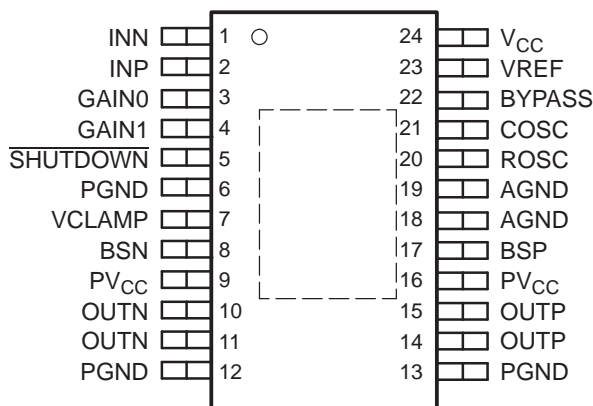
PWP PACKAGE (TOP VIEW)
