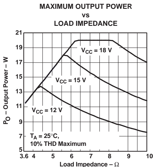
Figure 33. Output Power
