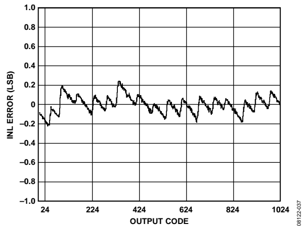
Figure 17. AD9204-80 INL with f_{IN} = 9.7 MHz
