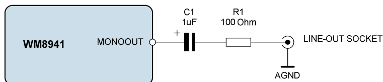
Figure 24 Recommended Circuit for Line Output
