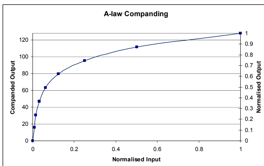
Figure 40 A-Law Companding
