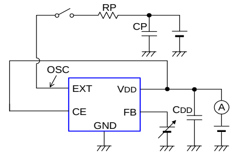
Circuit ④
