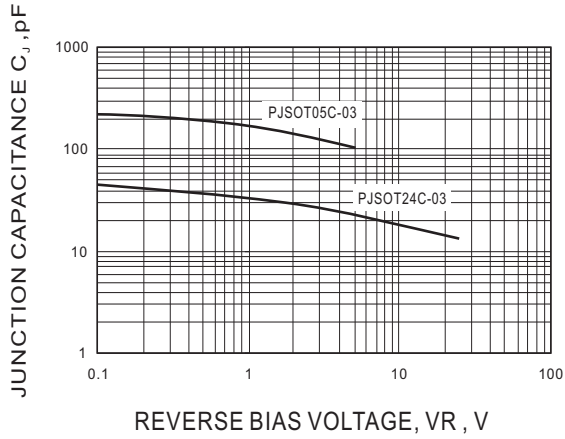
FIG. 1- TYPICAL CAPACITANCE
