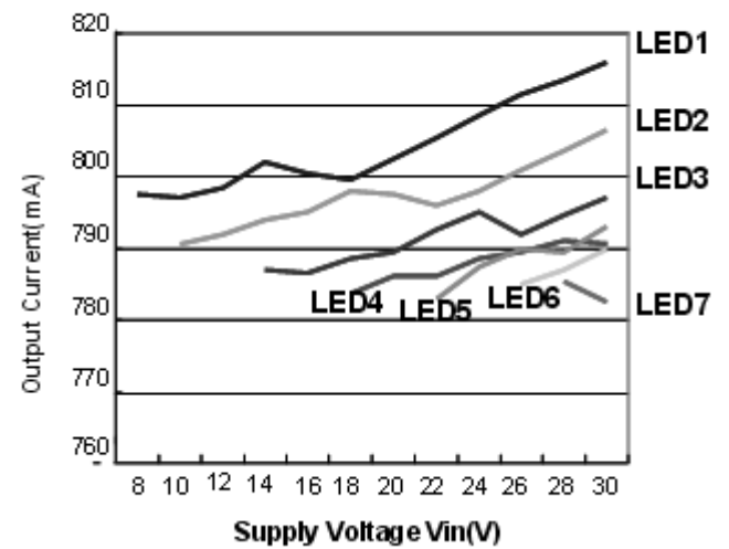
Output Current L=47\mu H R_{cs}=0.13\Omega
