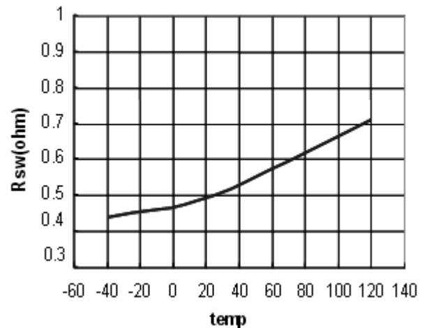
Rsw vs temperature, Vin=24V
