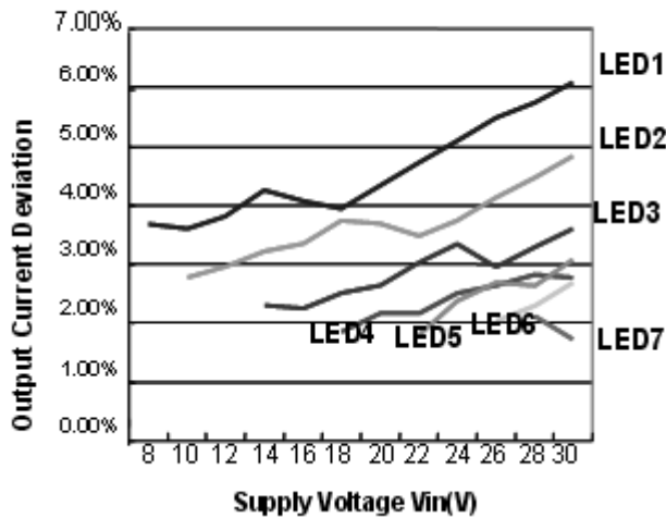
Output Current Deviation L=47\mu H R_{cs}=0.13\Omega
