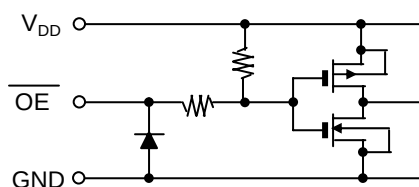
OEB Terminal
