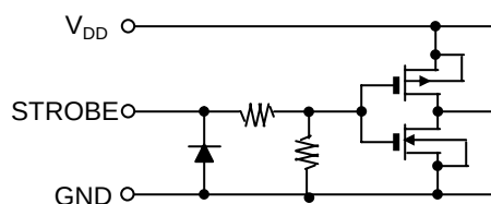
STROBE Terminal
