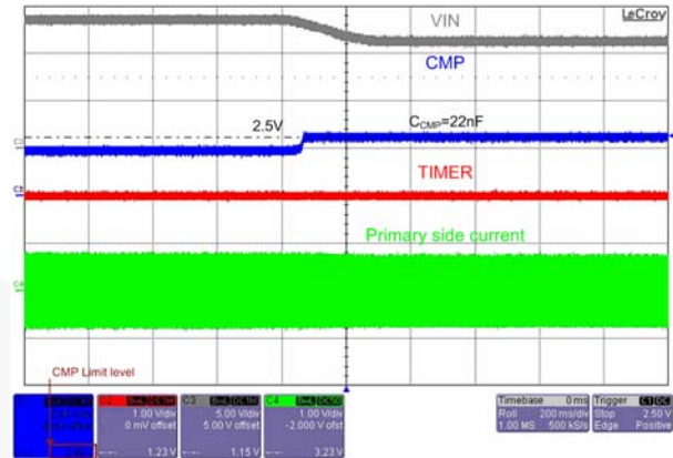
Figure 63. CMP-High Protection Disable by a Pull- Down Resistor
