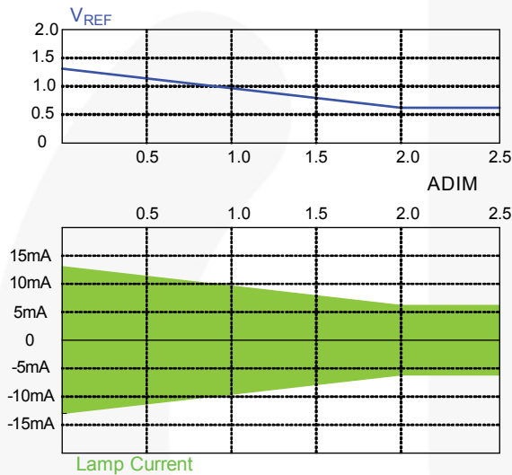
Figure 38. Analog Dimming Waveforms
