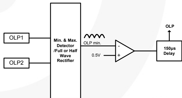
Figure 55. Open-Lamp Protection in Normal Mode
