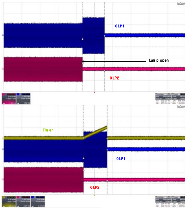
Figure 56. Open-Lamp Protection in Normal Mode
