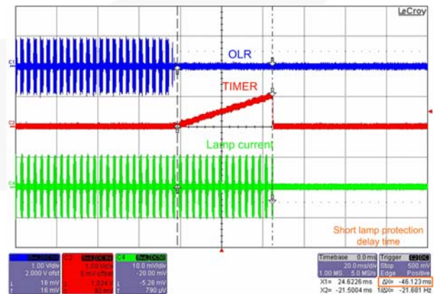
Figure 60. Short-Lamp Protection in Burst Dimming Mode
