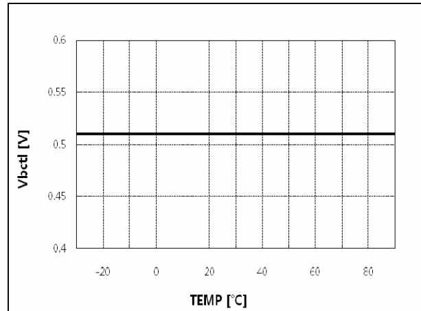
Figure 16. BCT Low Voltage vs. Temperature
