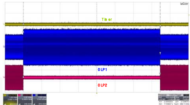
Figure 58. Open-Lamp Protection Disable in DCR Mode
