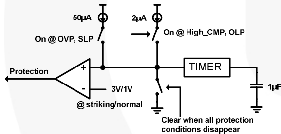
Figure 48. Protection Timing Delay
