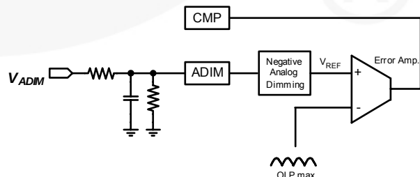
Figure 37. Analog Circuit Implementation
