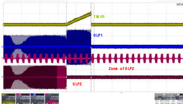
Figure 57. Open-Lamp Protection in Burst Dimming Mode
