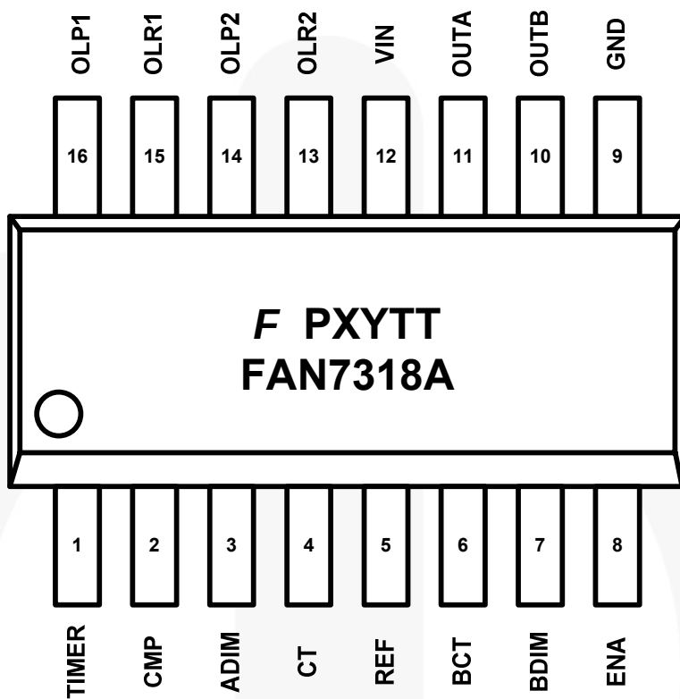
Figure 2. Package Diagram
