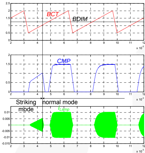
Figure 42. Burst Dimming During Striking Mode
