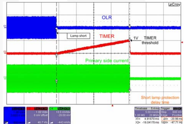
Figure 59. Short-Lamp Protection in Normal Mode
