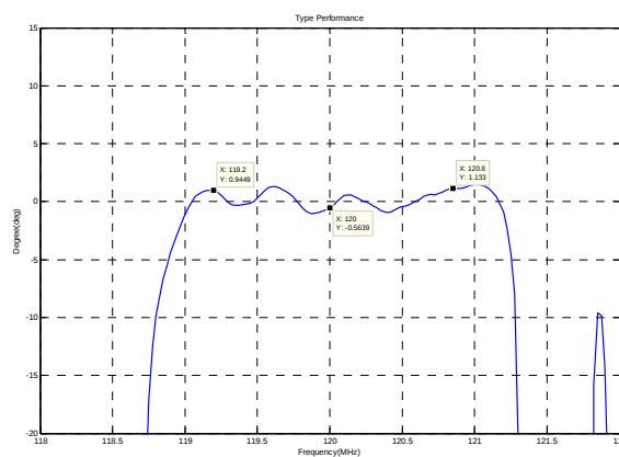
Phase Linearity( f_0 \pm 0.8\text{MHz} )
