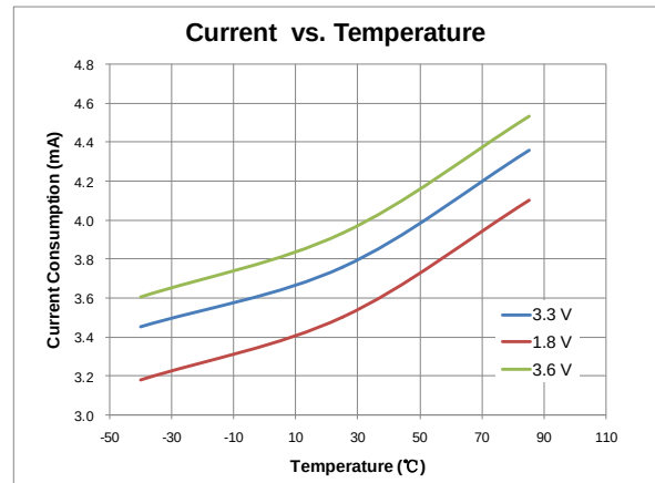
Figure 4. Current vs. Temperature, F_{RF} = 433.92 MHz, SR = 1 kps
