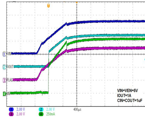
Startup from Power ON (WS4611A)
