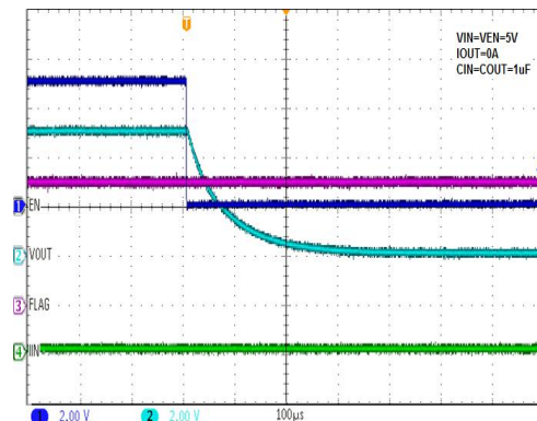
Shutdown from Enable OFF (WS4611A)
