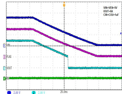
Shutdown from Power OFF (WS4611A)
