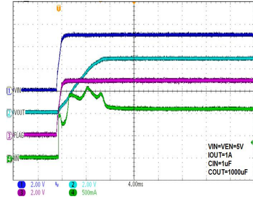
Startup from Power ON (WS4611A)
