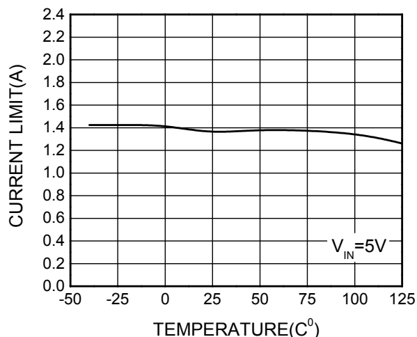
Current Limit vs. Temperature (WS4611A)
