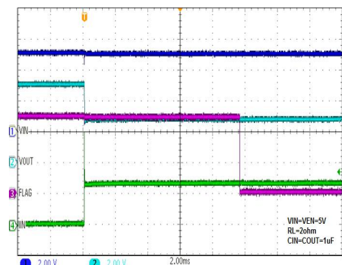
Current Limit Response (WS4611A)
