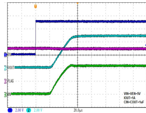
Startup from Enable ON (WS4611A)
