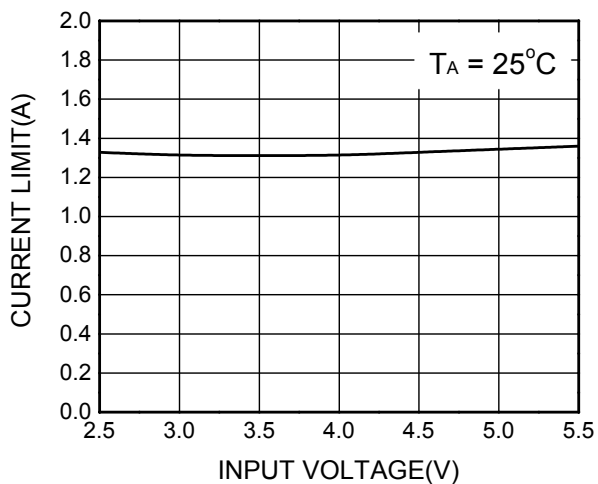
Current Limit vs. Input Voltage (WS4611A)
