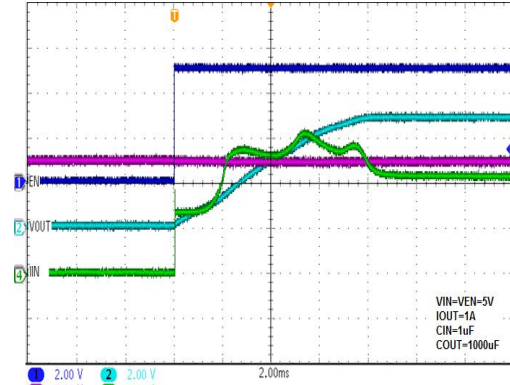
Startup from Enable ON (WS4611A)
