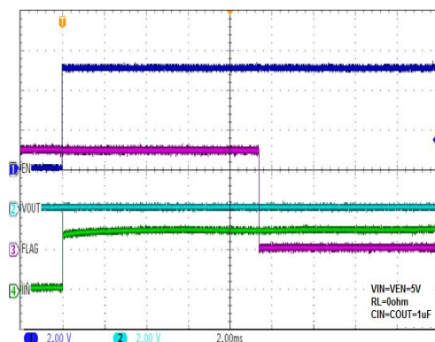
Start into Short Circuit (WS4611A)
