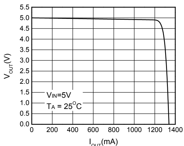
Output Voltage vs. Output Current (WS4611A)
