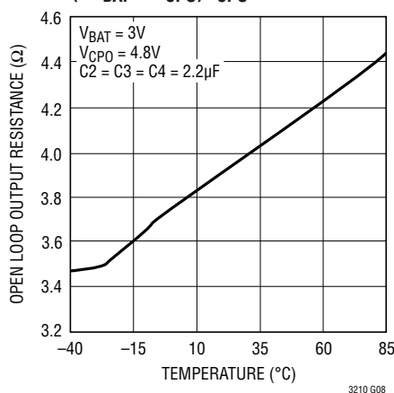
2x Mode Charge Pump Open-Loop Output Resistance vs Temperature (2V_{BAT} - V_{CP0})/I_{CPO}
