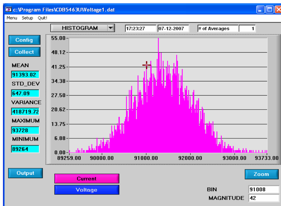
Figure 14. Histogram Analysis
