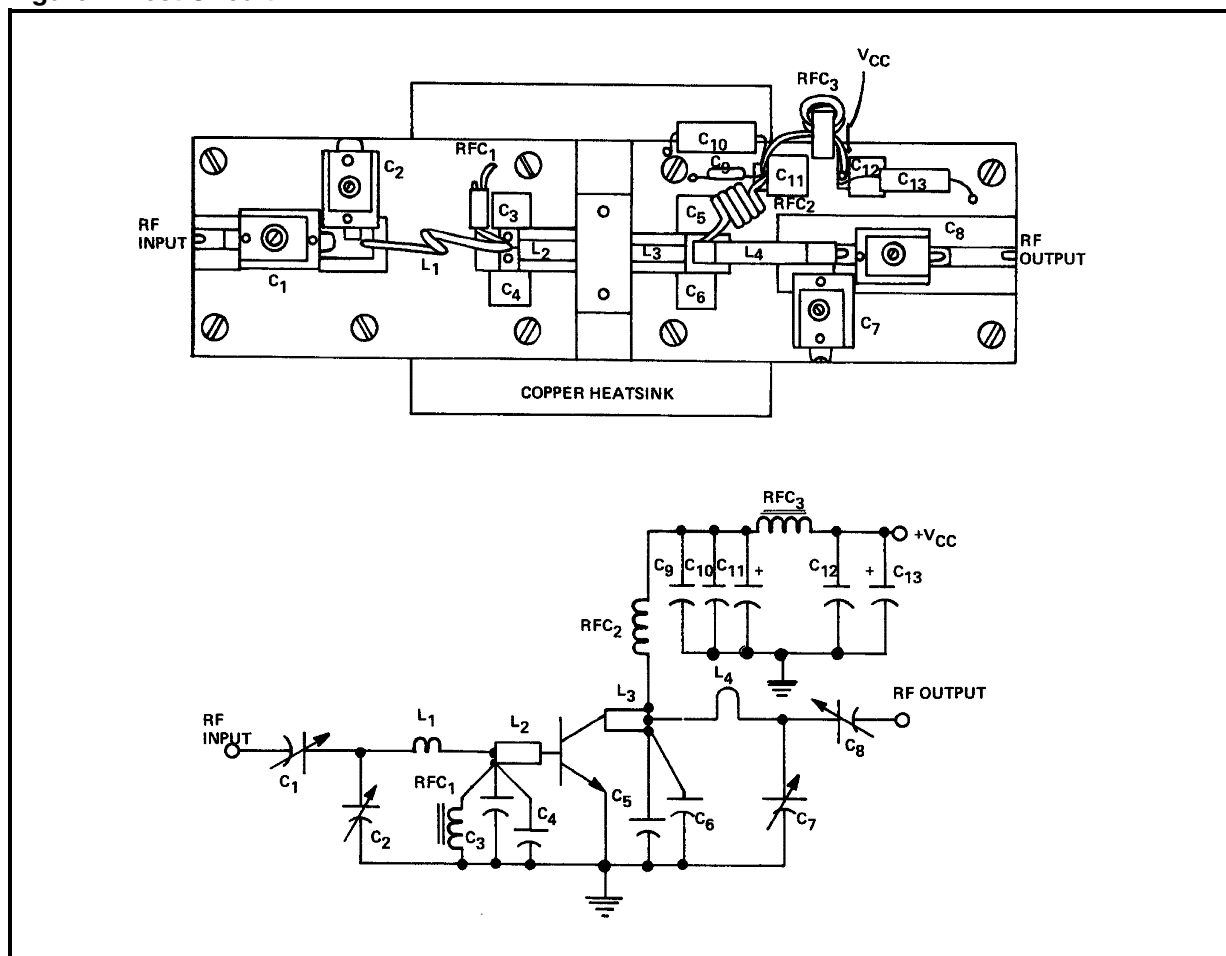
Figure 7. Test Circuit
