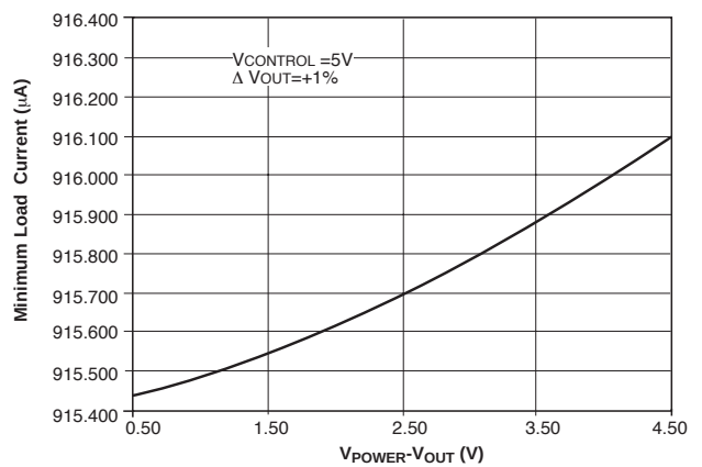
Minimum Load Current vs V_{\text{POWER}} - V_{\text{OUT}}
