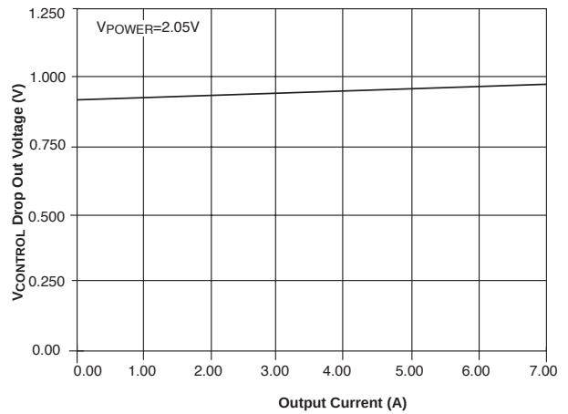
V_{\text{CONTROL}} Dropout Voltage vs I_{\text{OUT}}
