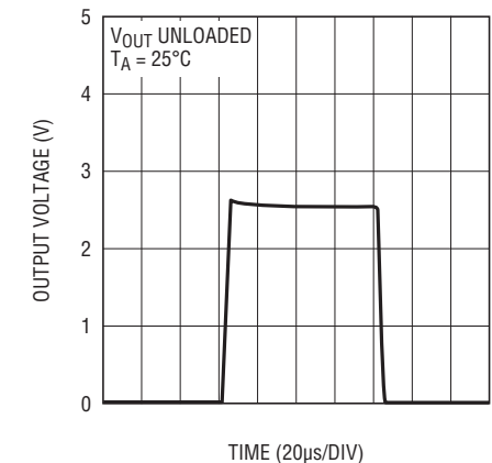
LTC1657L Large-Signal Transient Response
