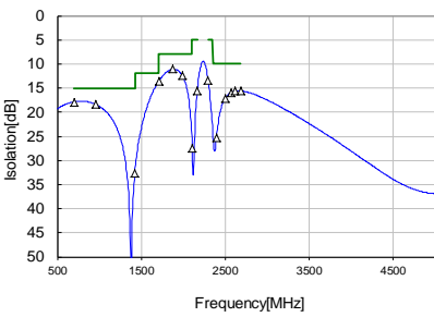
Isolation
