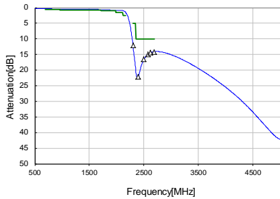
Low band-Port
