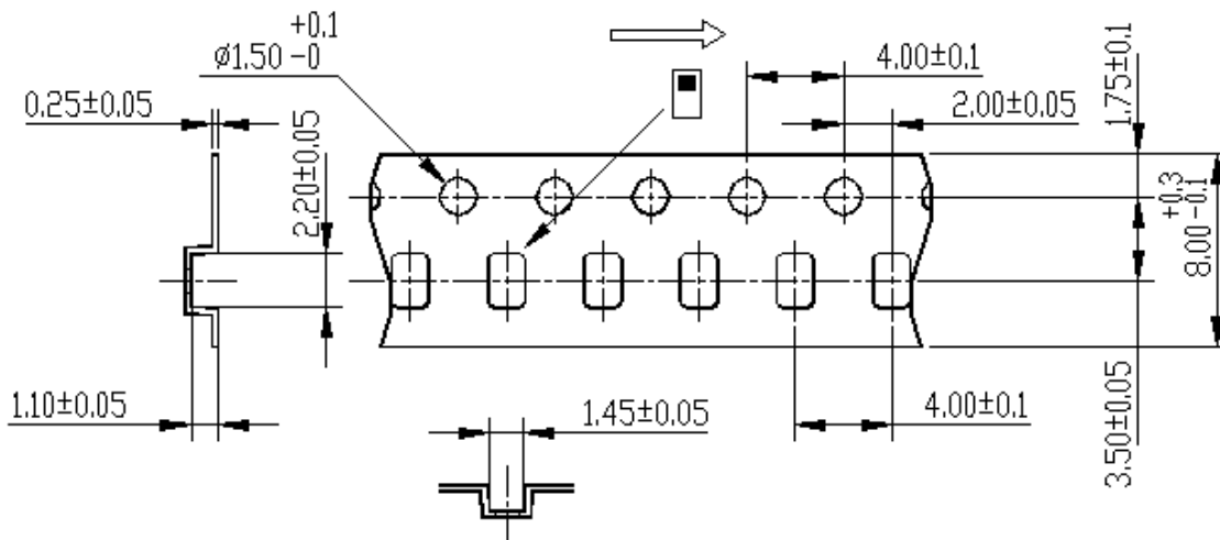
Carrier Tape
