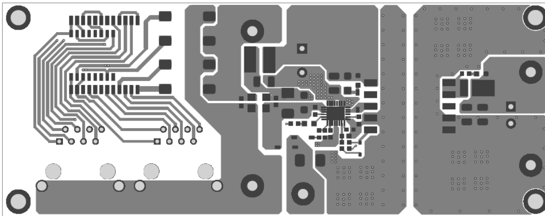
Figure 2: Top Layer
