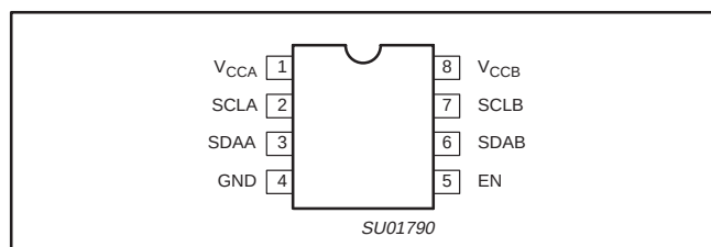
Figure 1. Pin configuration
