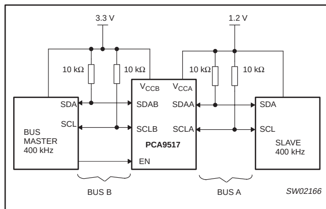
Figure 3. Typical application
