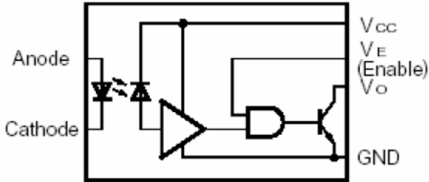
Circuit Block Diagram
