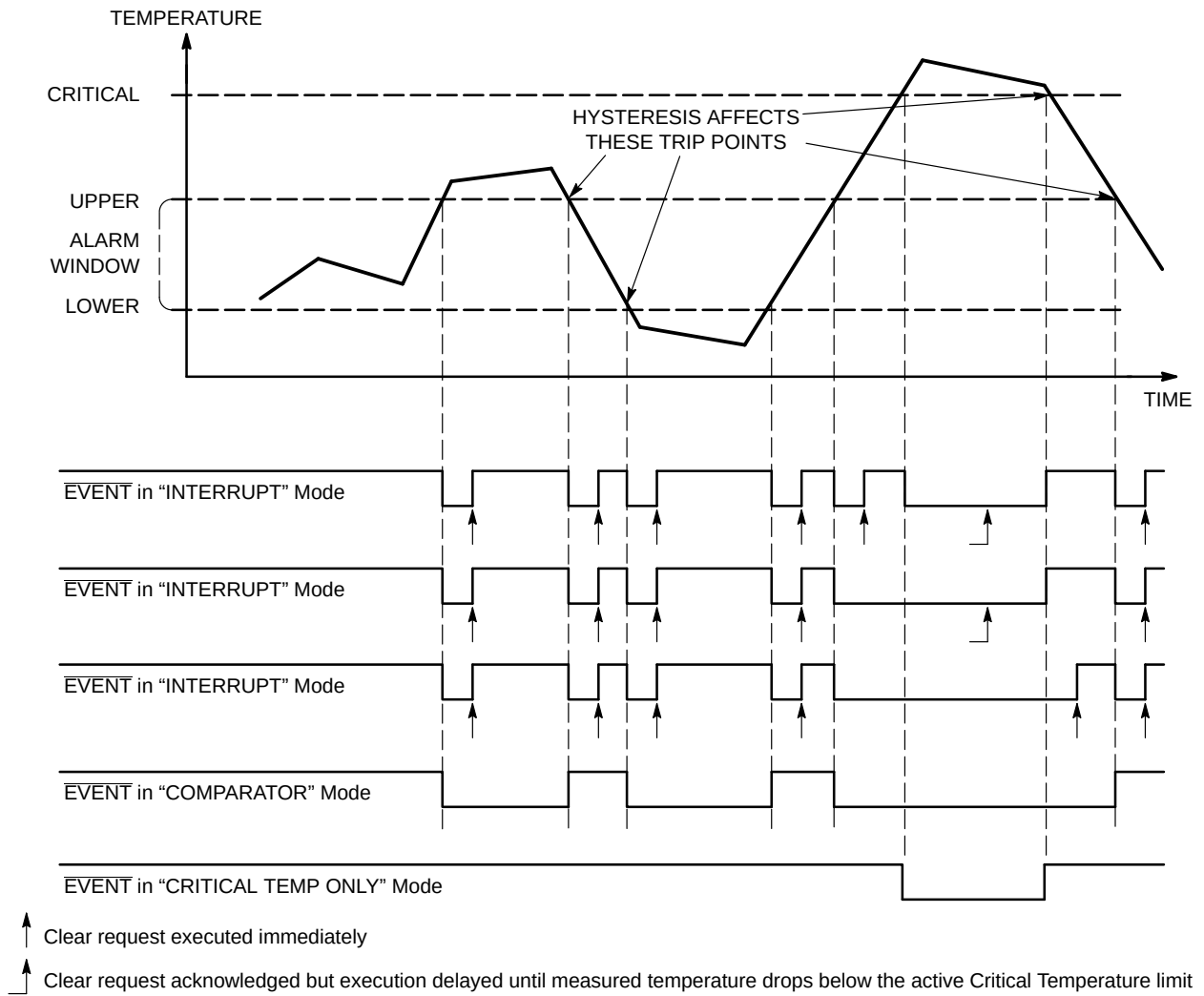
Figure 9. Event Detail
