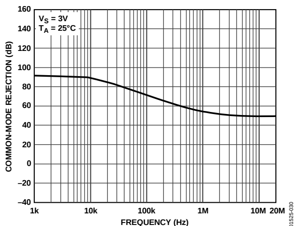
Figure 30. Common-Mode Rejection Ratio vs. Frequency
