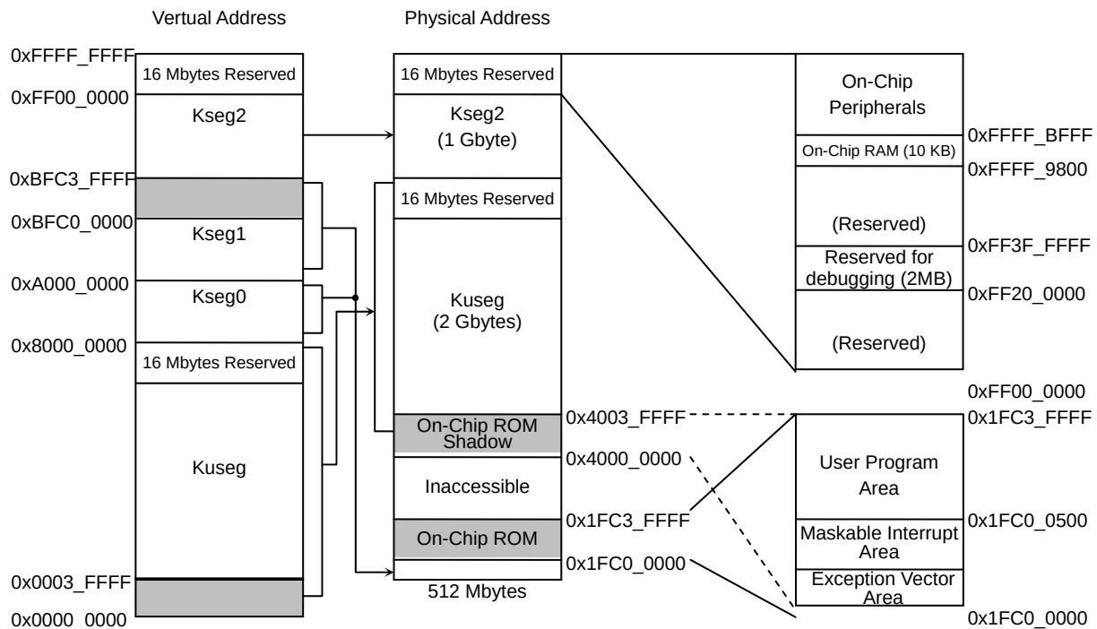
Figure 4.1.1 Memory Map
