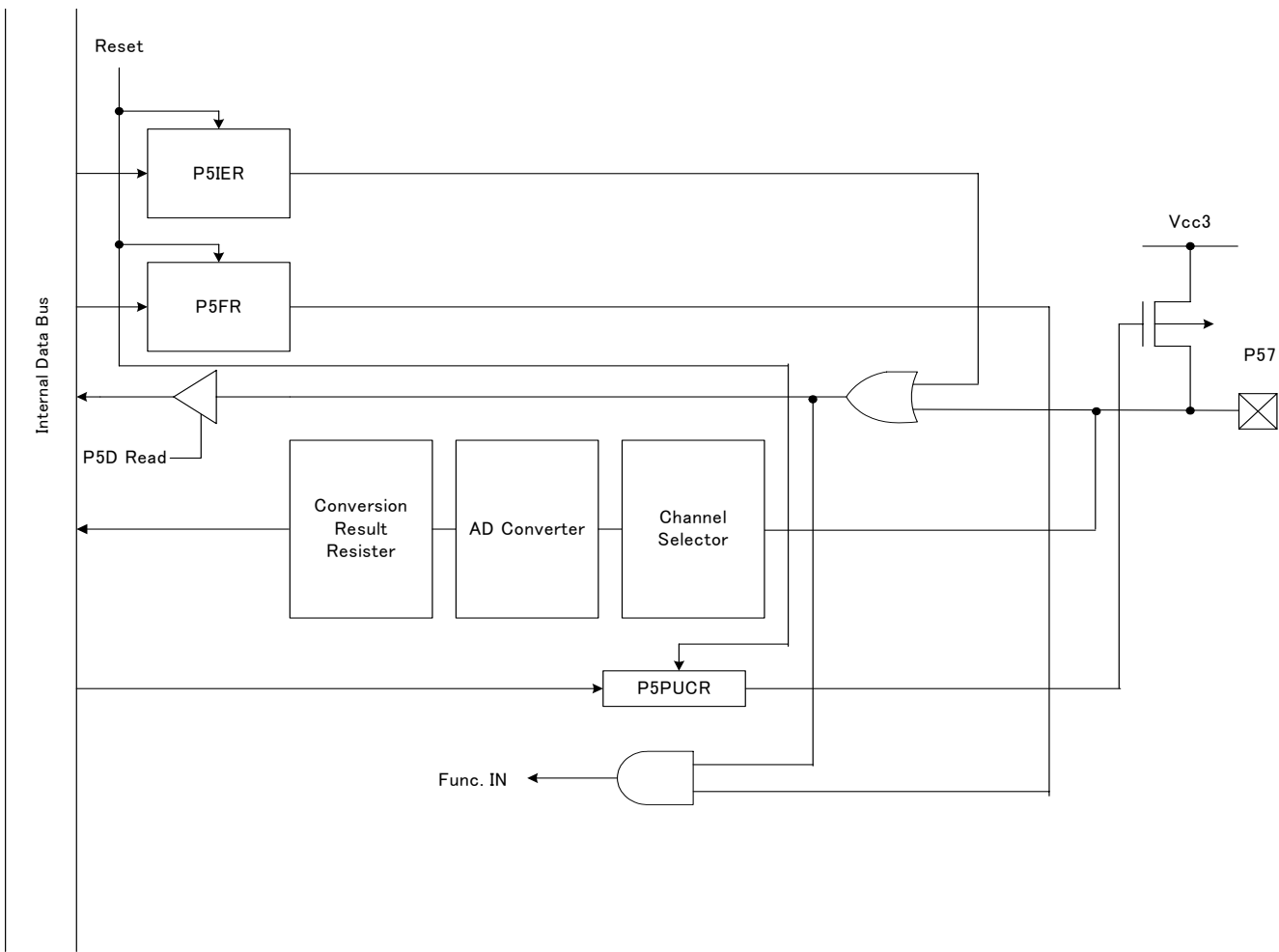
Figure 8.5.2 Port 5 (P57)
