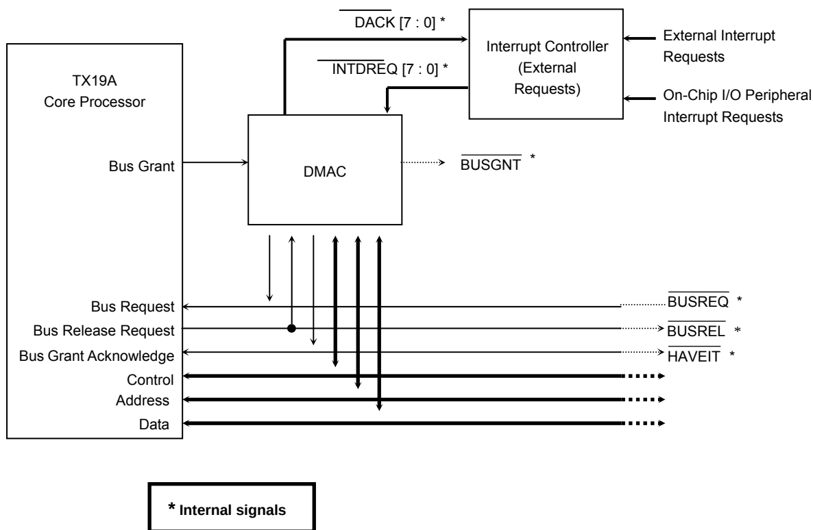
Figure 10.2.1 DMAC Connections within the TMP19A71
