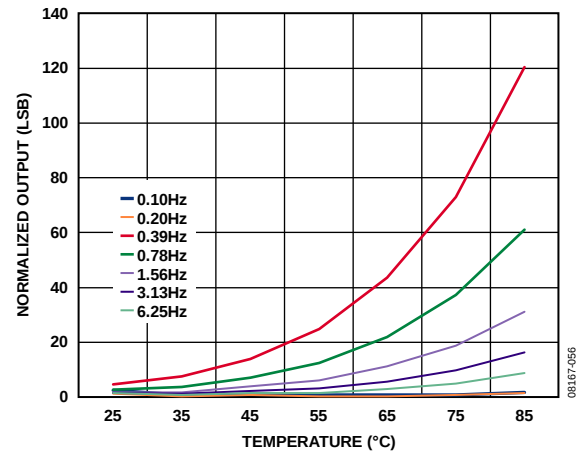
Figure 56. Typical X-Axis Output vs. Temperature at Lower Data Rates, Normalized to 100 Hz Output Data Rate, V_S = 2.6\text{ V}
