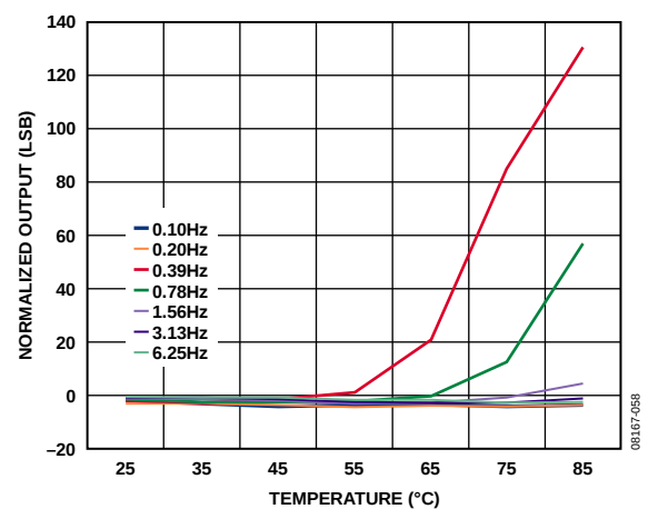
Figure 58. Typical Z-Axis Output vs. Temperature at Lower Data Rates, Normalized to 100 Hz Output Data Rate, V_S = 2.6\text{ V}
