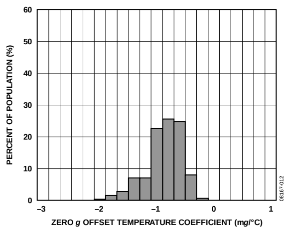
Figure 12. Z-Axis Zero g Offset Temperature Coefficient, V_S = 2.6\text{ V}
