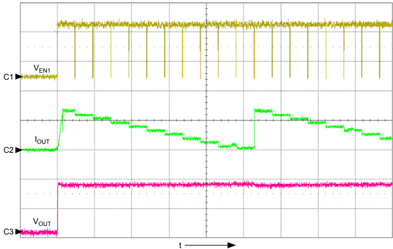
11-Level Single-Wire Serial Dimming Response
