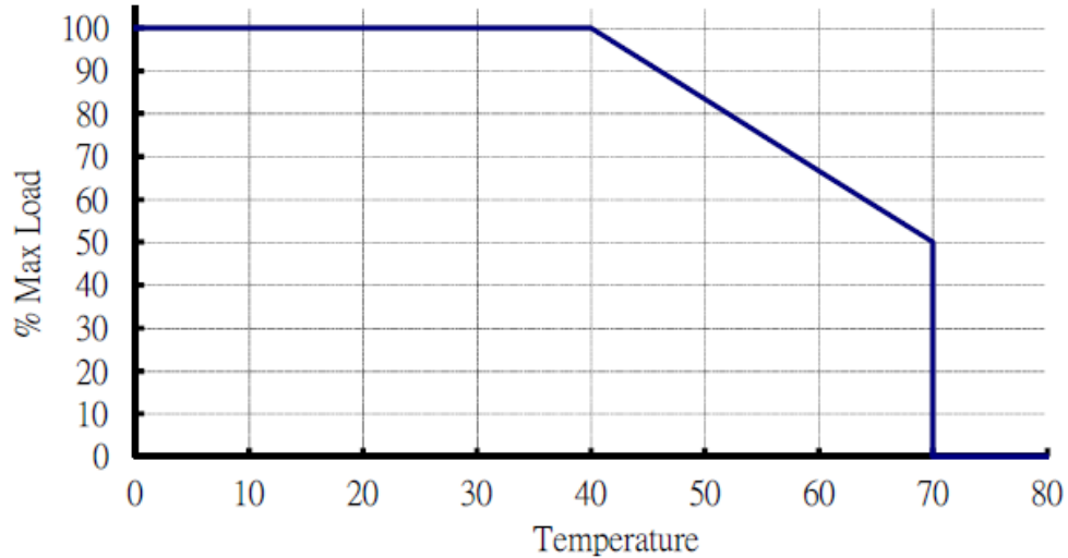
Derating Curve
