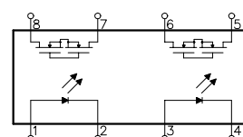
DUAL 1 FORM B NORMALLY CLOSE
