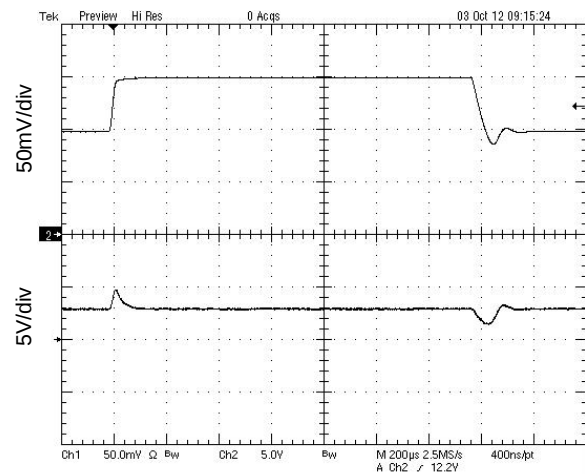
Figure 9. Line Transient Response ( V_{CC}=12\text{V} , V_{OUT}=3.3\text{V} )
