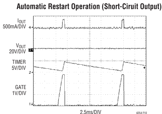
Figure 10. RETRY Waveforms
