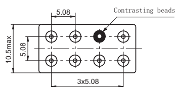
Mouting style 0
