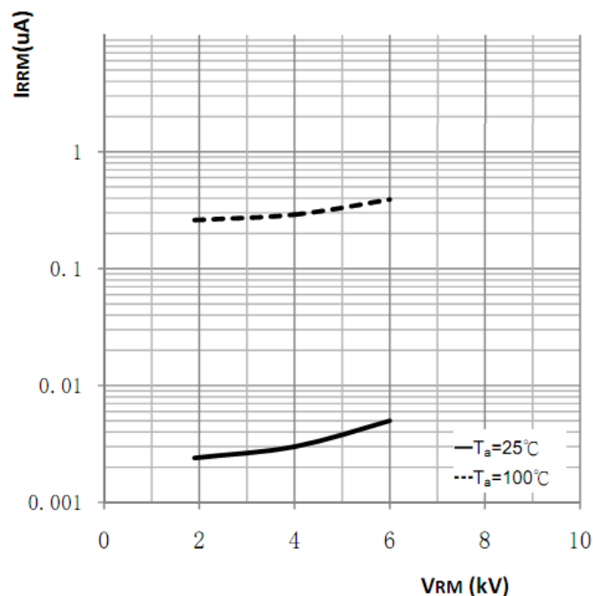
Reverse Characteristics
