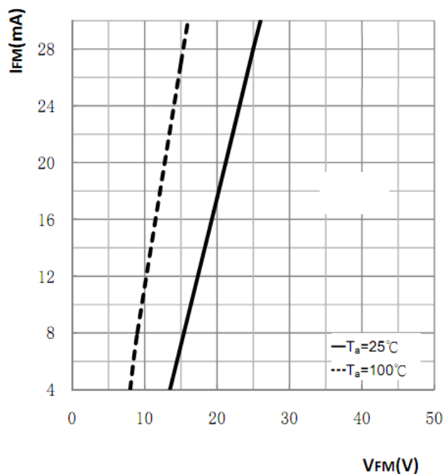
Forward Characteristics
