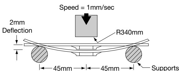
Figure 2. Bend Strength
