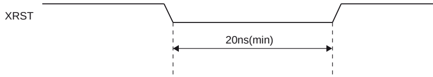
Lo period restriction of XRST pin
