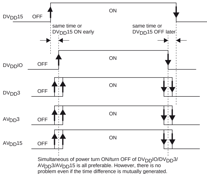
Power turn-ON/turn-OFF sequence
