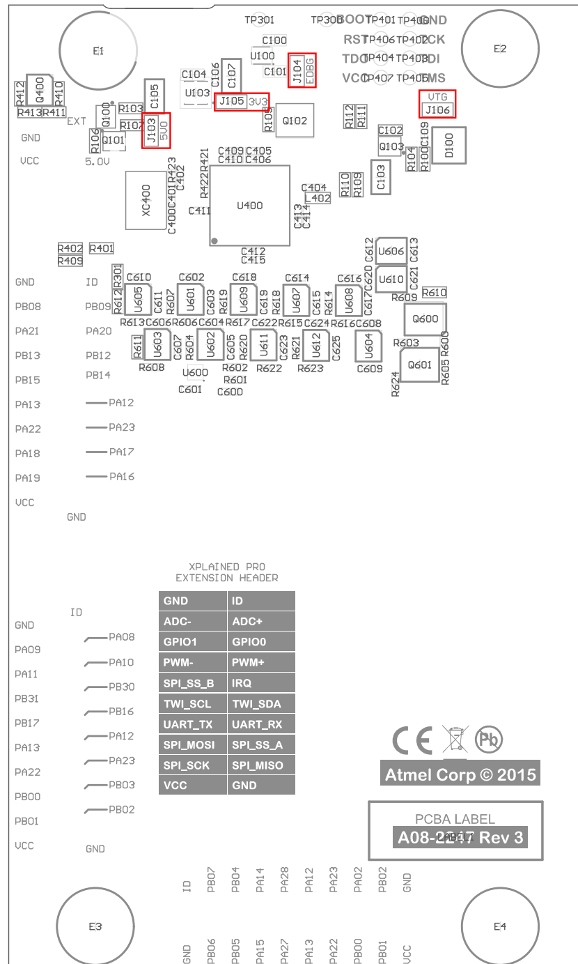
Figure 4-6. Jumpers Bottom
