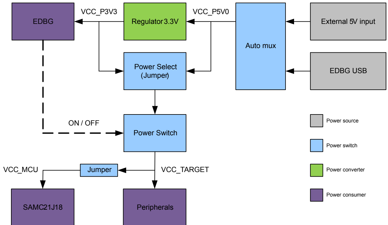
Figure 6-1. Revision 2 and 3 Power Supply Block Diagram
