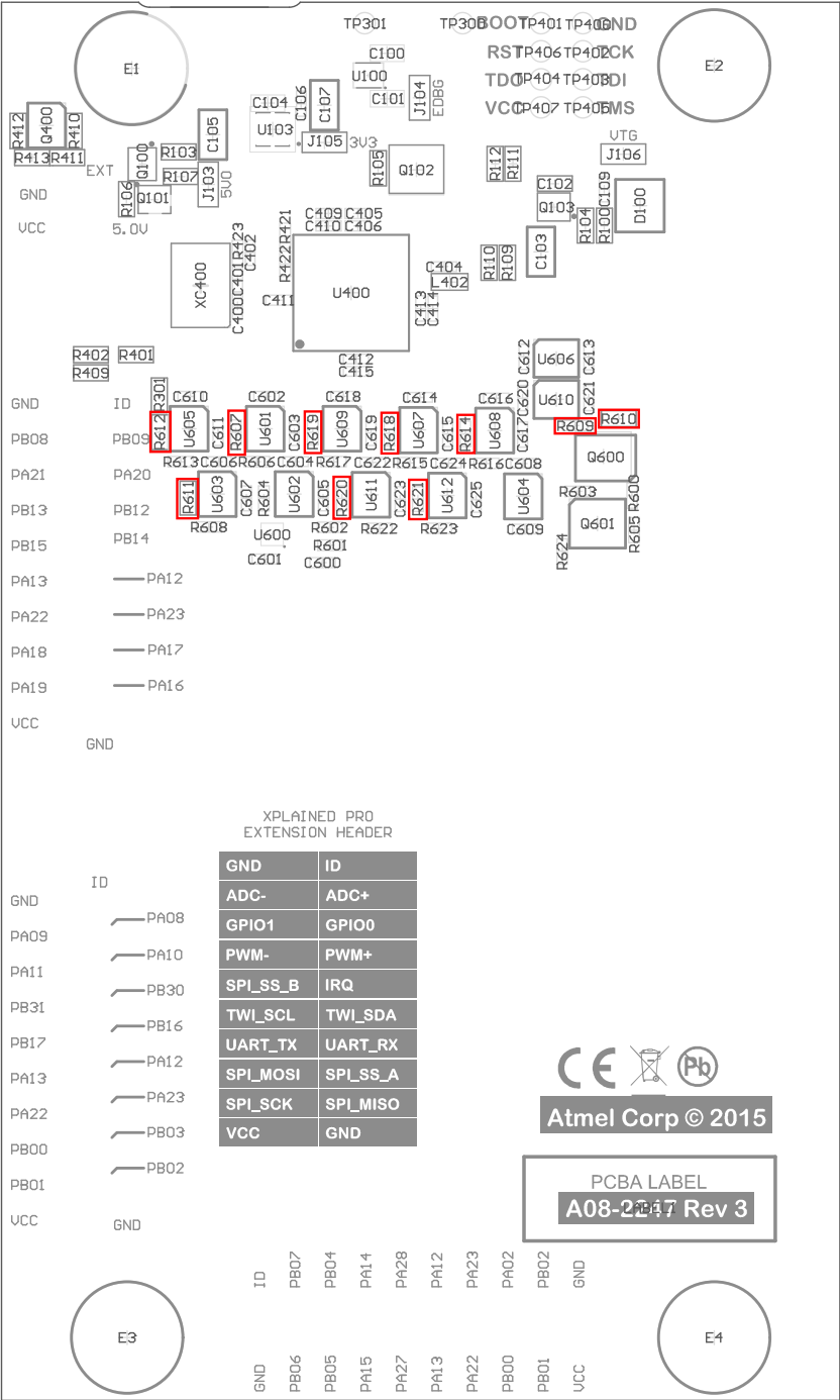
Figure 4-4. Resistors Bottom
