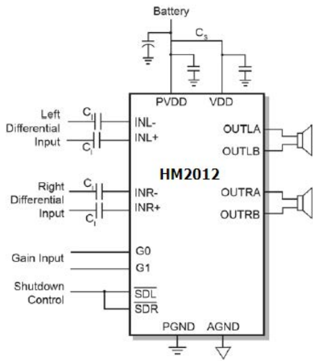
Figure5. Differential Input
