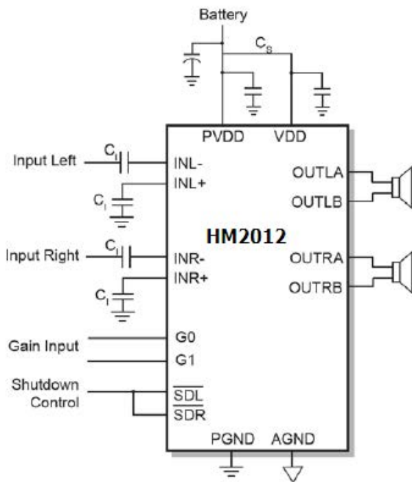
Figure4. Single-ended Input
