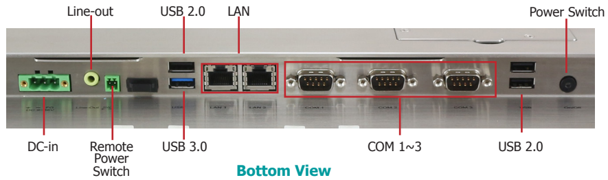
Bottom View
