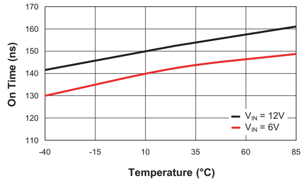
Switching Current vs. Temperature ( V_{OUT} = 5V )
