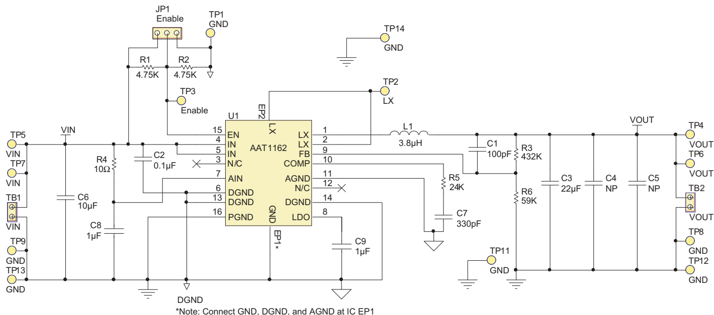
Figure 2: AAT1162 Evaluation Board Schematic.
