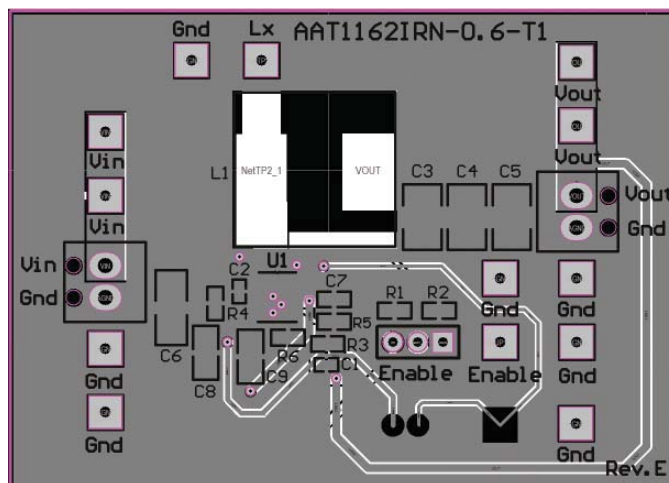
Figure 4: AAT1162 Evaluation Board Solder Side Layout.
