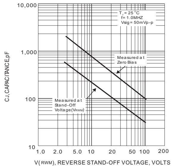
Fig.4 TYPICAL CAPACITANCE
