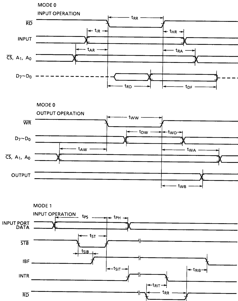
Figure 7.1 Timing diagram
