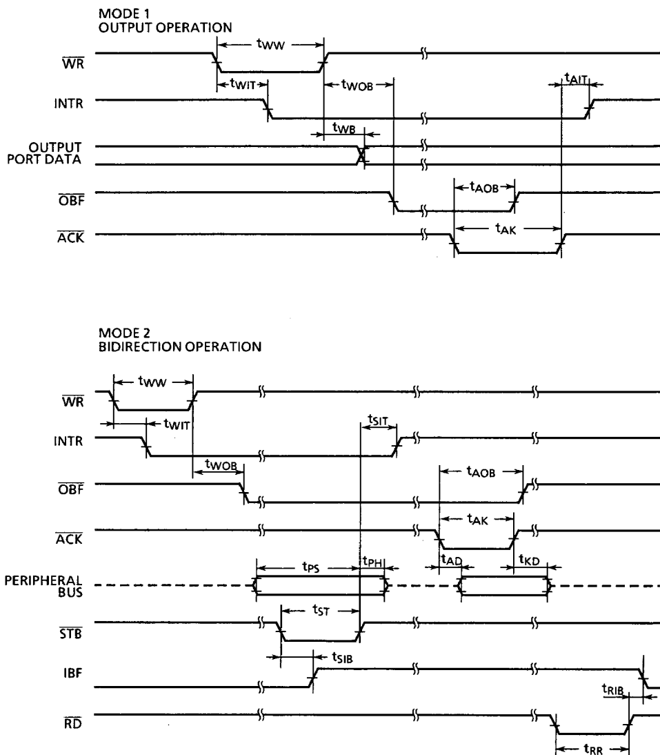
Figure 7.2 Timing diagram
