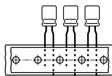
Case \varnothing D = 5 to 8 mm; pitch F is 5 mm
