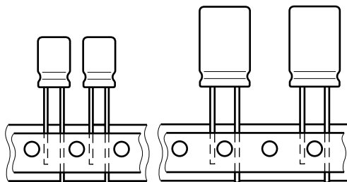
Dimensions of pitch F see tables 1 and 2
