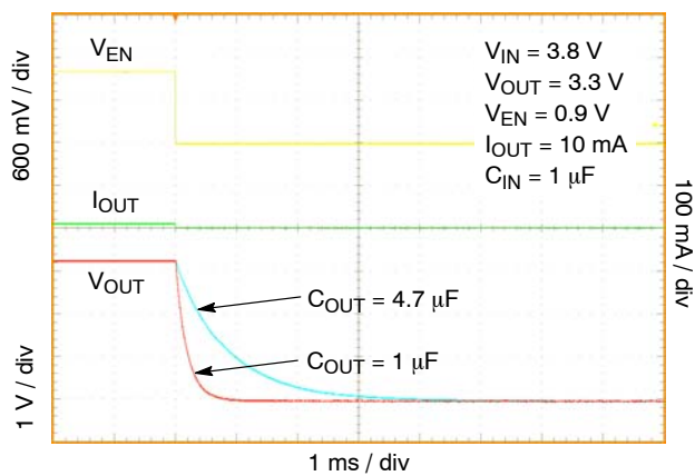
Figure 38. Enable Turn-off Response
