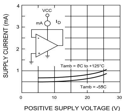
Figure 13: Supply current
