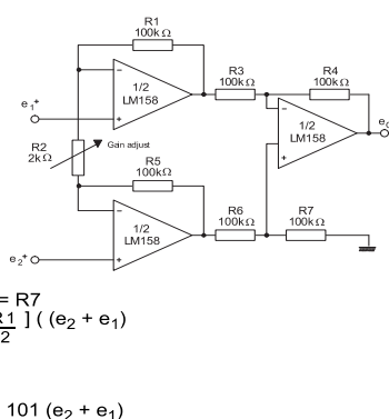
Figure 24: High input Z adjustable gain DC instrumentation amplifier
