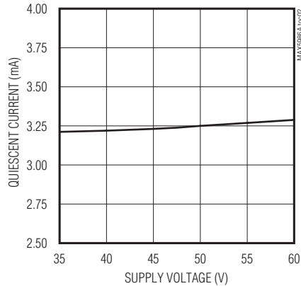
QUIESCENT CURRENT vs. SUPPLY VOLTAGE (ULTRA-LOW POWER MODE)
