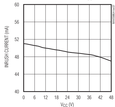
INRUSH CURRENT LIMIT vs. V_{CC} VOLTAGE
